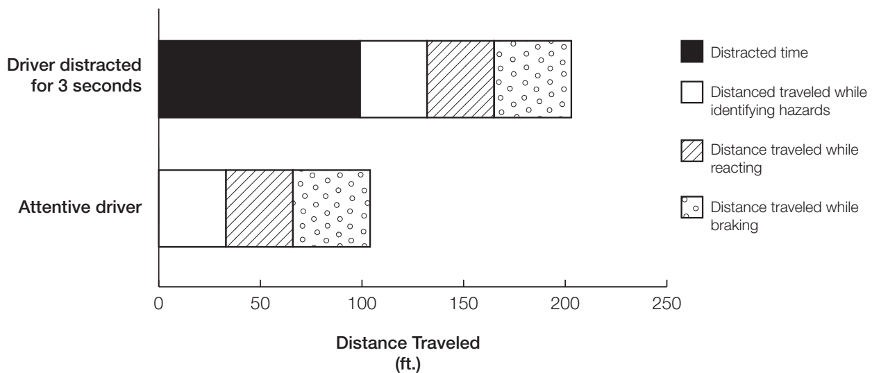
Figure 1. Distance Needed to Stop: Distracted Drivers vs. Attentive Drivers
